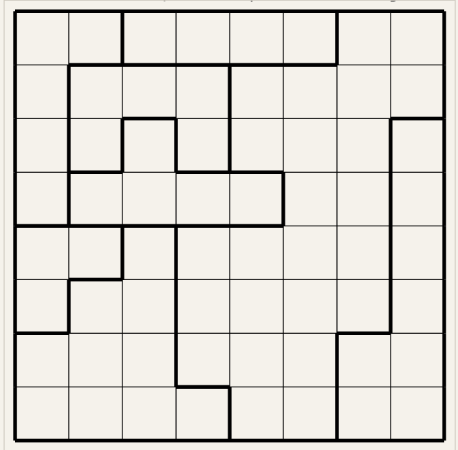
Puzzle 4 (8×8, 1 star per row/col/region)
