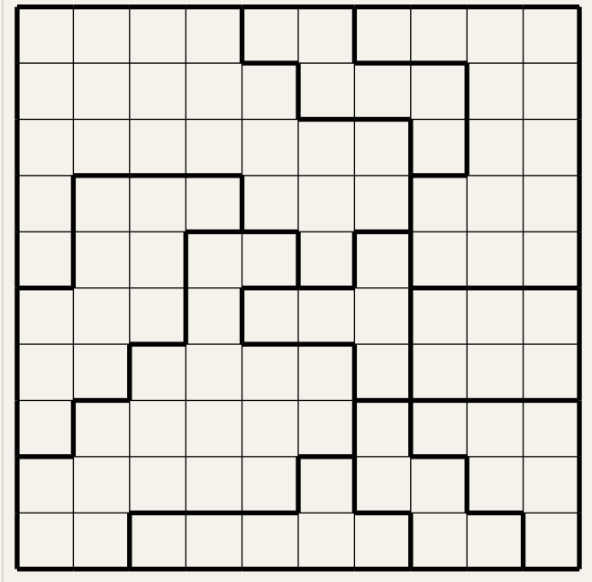
Puzzle 6 (10×10, 1 star per row/col/region)
