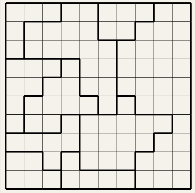
Puzzle 8 (10×10, 1 star per row/col/region)
