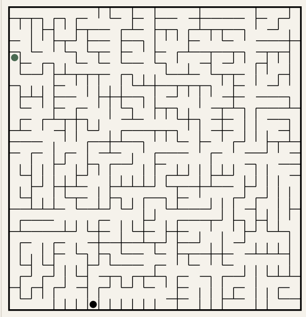
Puzzle 1 (26x27)
