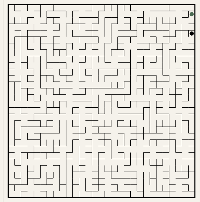
Puzzle 2 (29x30)
