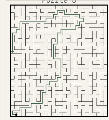
Puzzle 8
