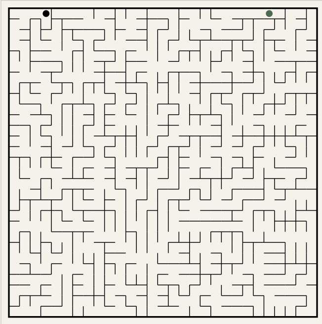
Puzzle 1 (29x29)
