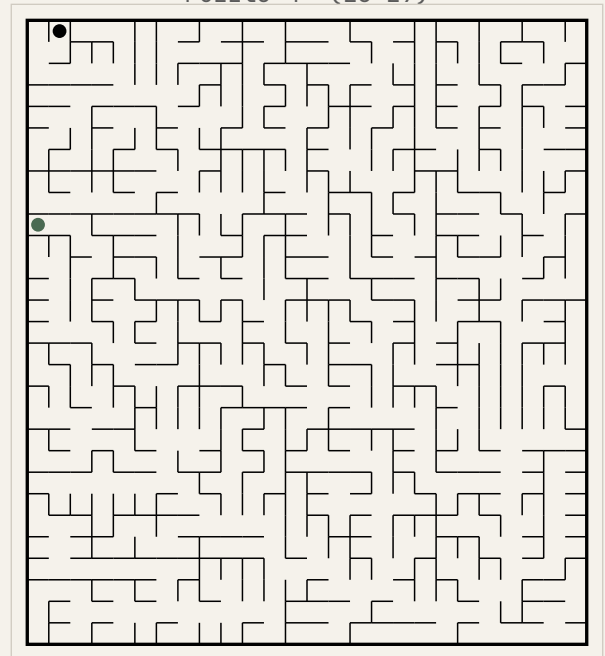
Puzzle 4 (26x29)
