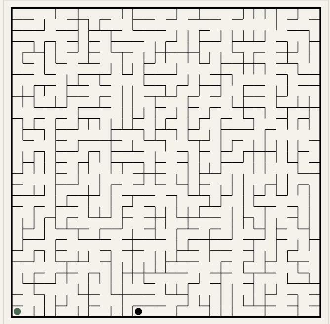
Puzzle 2 (28x28)
