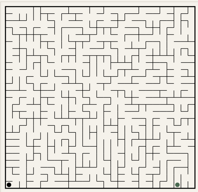
Puzzle 3 (27x26)
