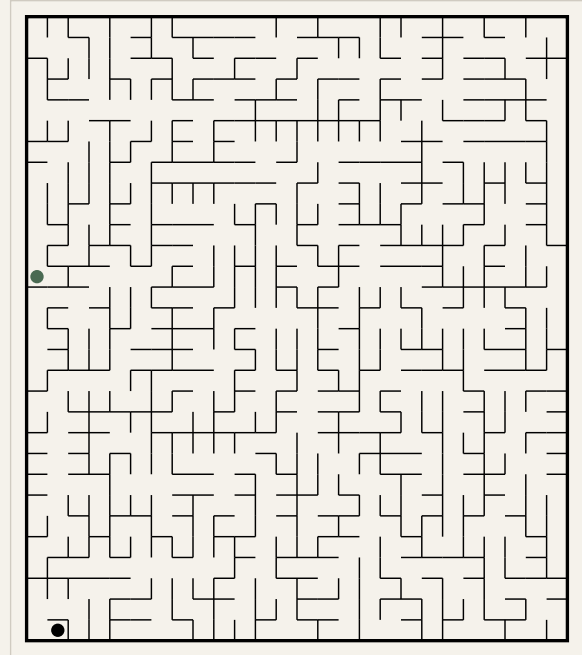
Puzzle 6 (26x30)
