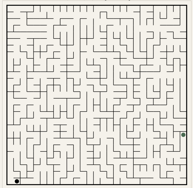
Puzzle 8 (27x27)
