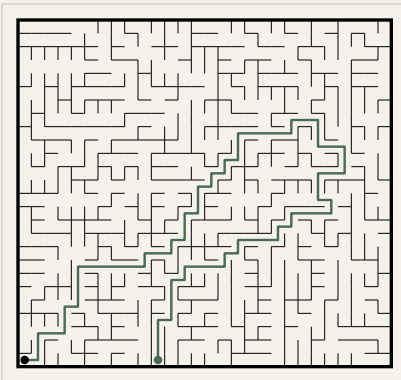
Puzzle 7
