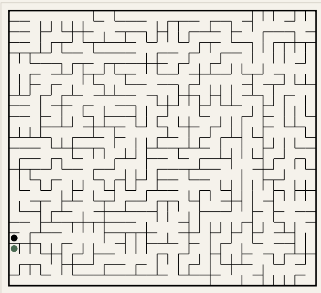
Puzzle 3 (29x26)
