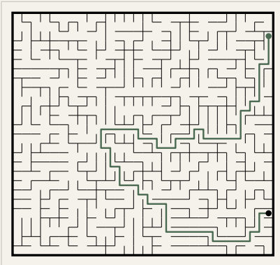
Puzzle 5
