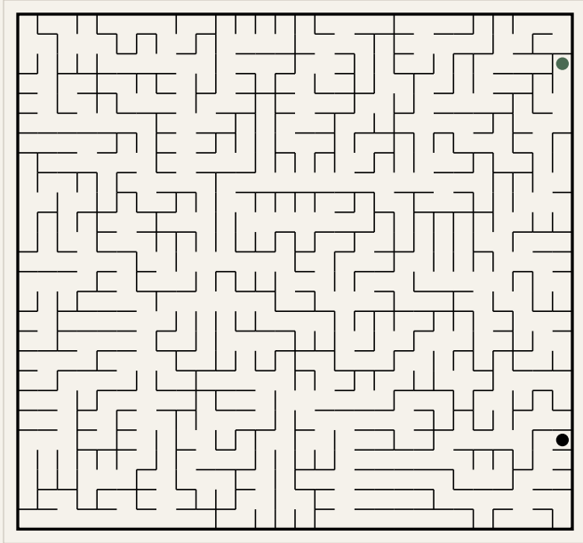
Puzzle 5 (28x26)
