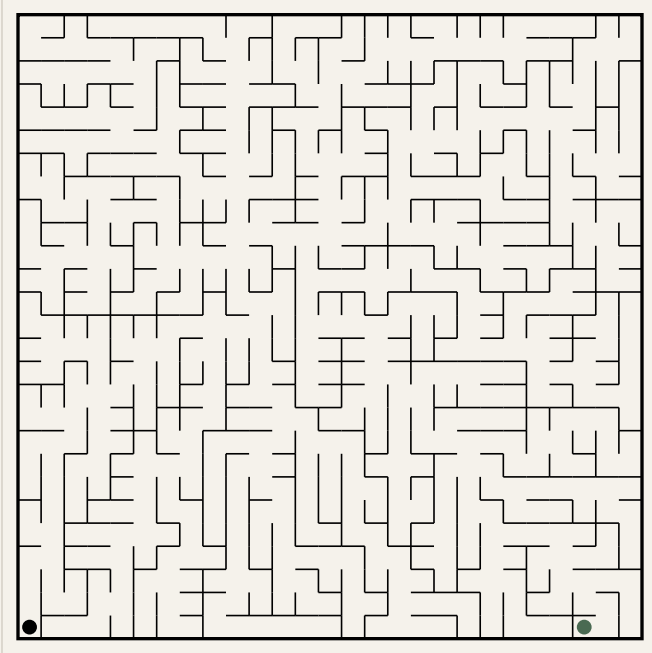
Puzzle 1 (27x27)
