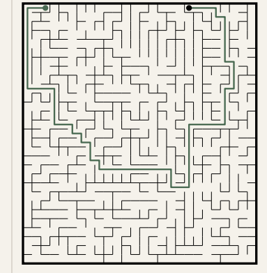
Puzzle 8
