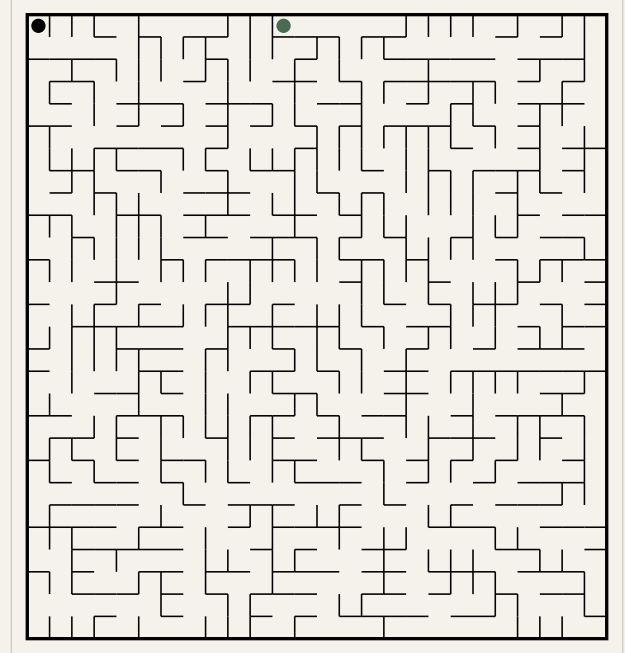
Puzzle 2 (26x28)
