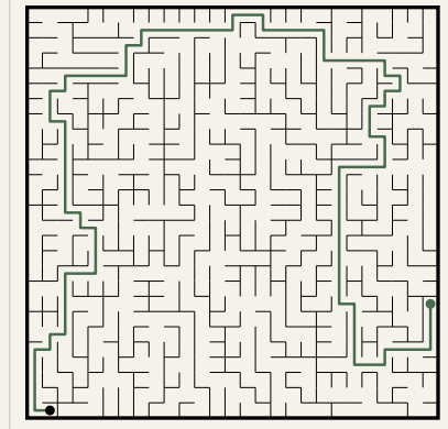
Puzzle 8
