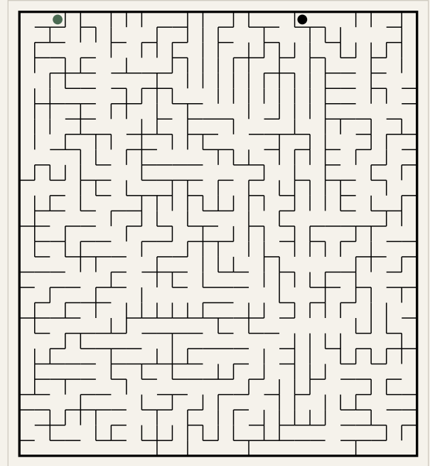
Puzzle 6 (26x29)
