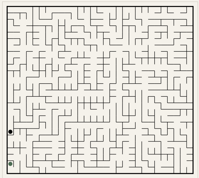
Puzzle 4 (29x26)
