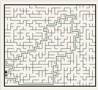
Puzzle 3
