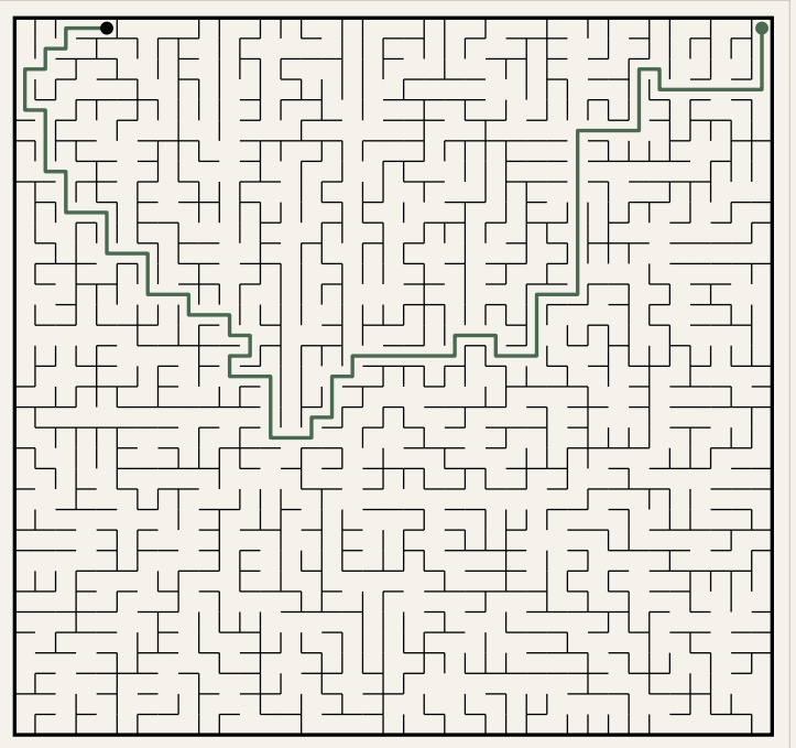
Puzzle 2
