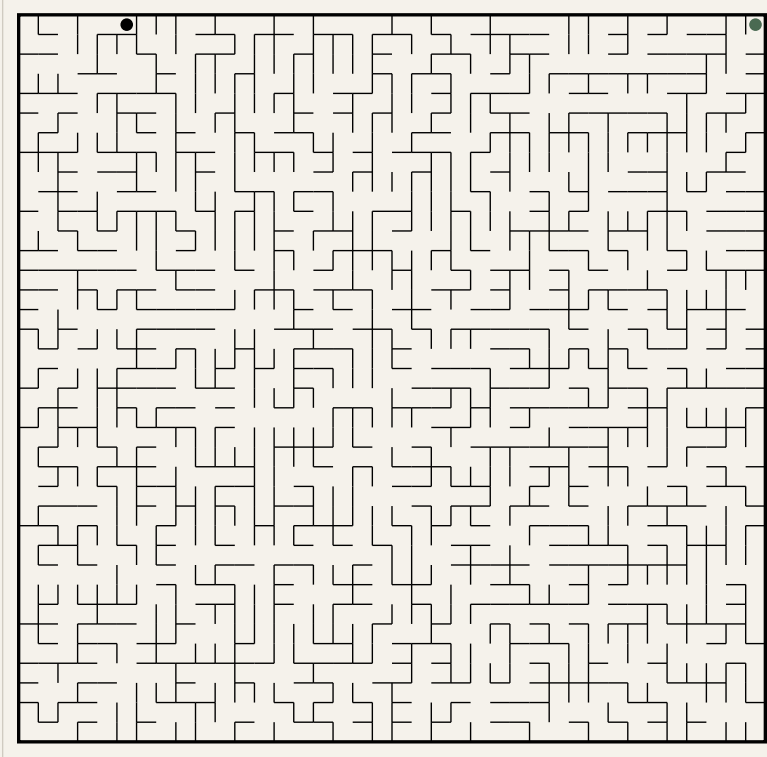
Puzzle 1 (38×37)
