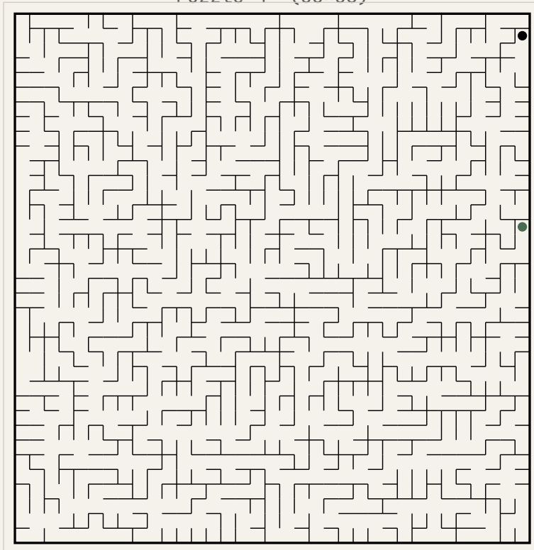
Puzzle 4 (35x36)
