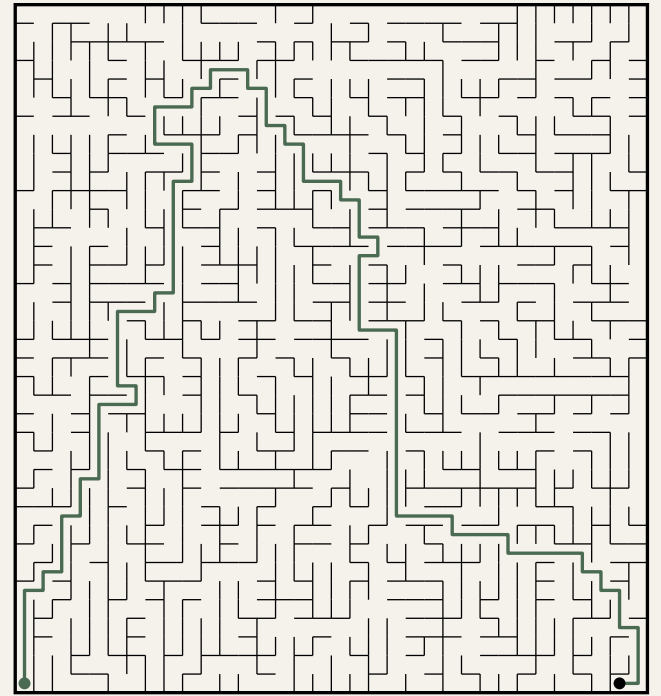
Puzzle 2
