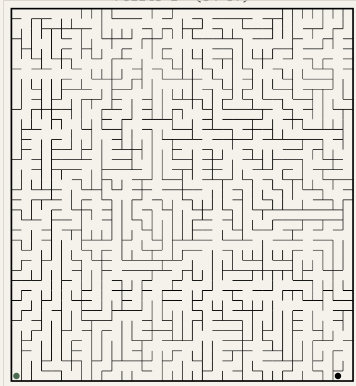
Puzzle 2 (34x37)
