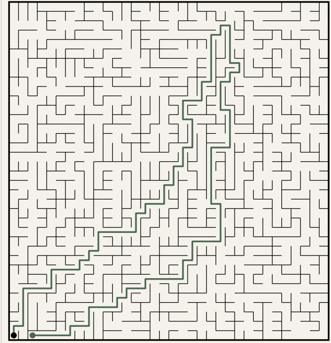
Puzzle 4
