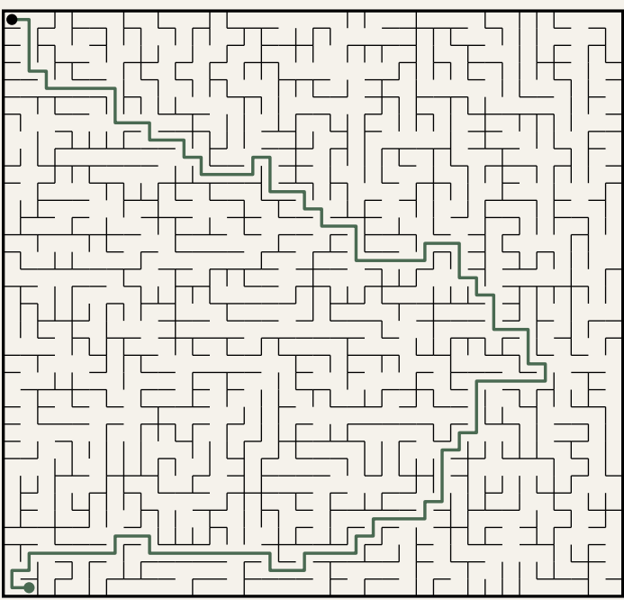
Puzzle 3
