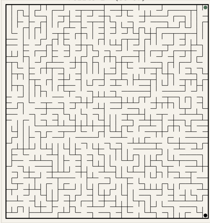
Puzzle 1 (35x37)
