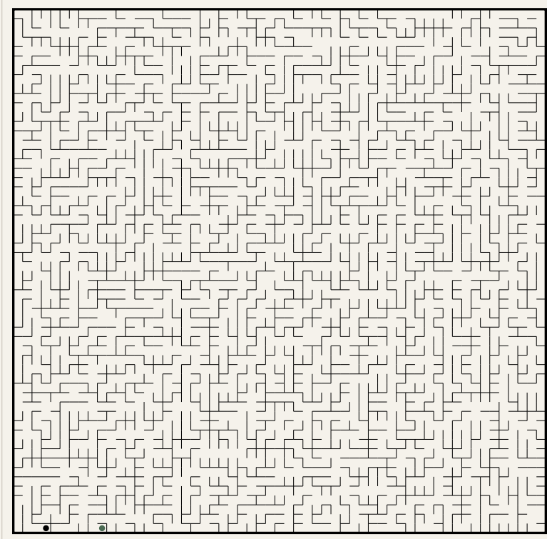
Puzzle 2 (57x56)
