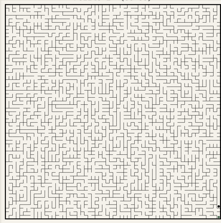
Puzzle 1 (60x60)
