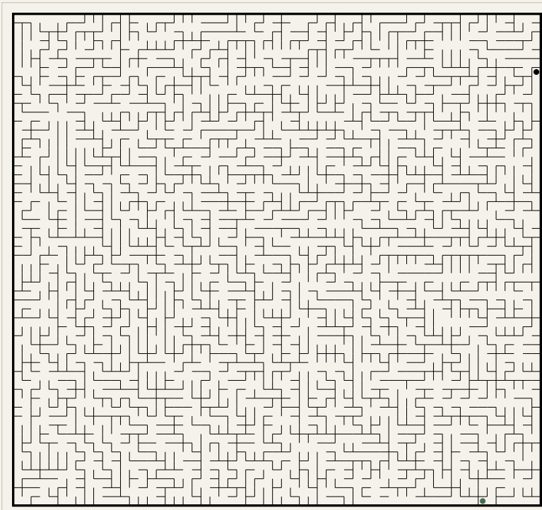
Puzzle 2 (59x55)
