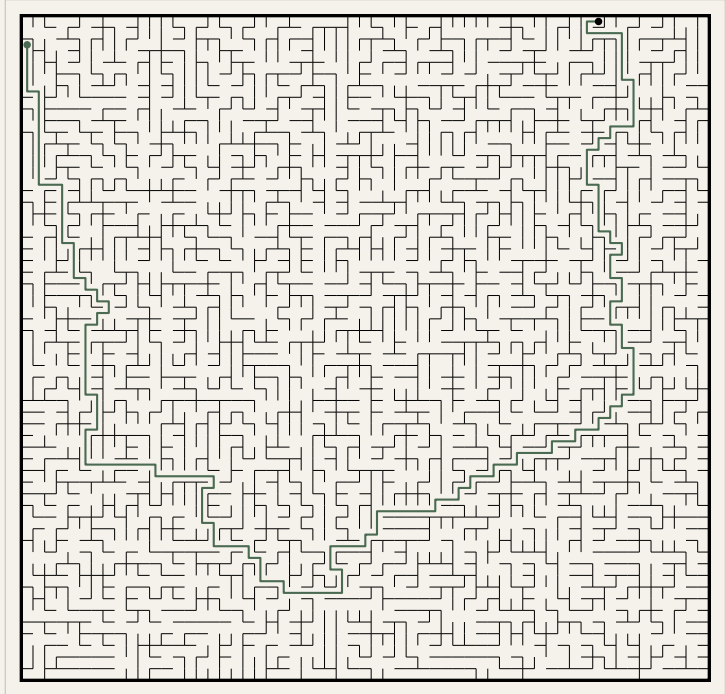
Puzzle 4
