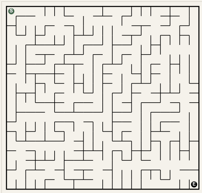
Puzzle 7 (20x19)
