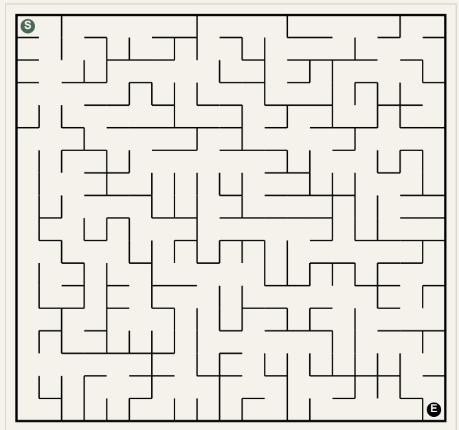
Puzzle 8 (19x18)
