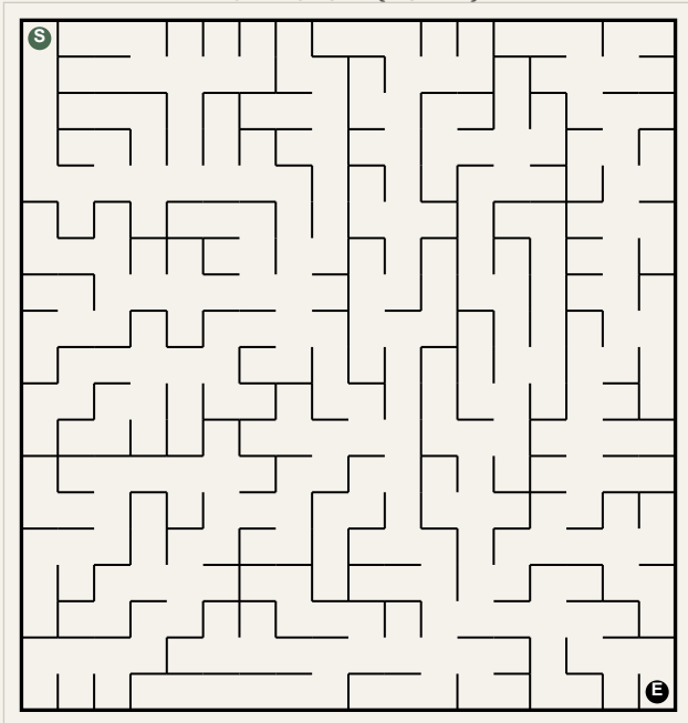
Puzzle 3 (18x19)
