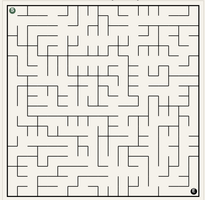
Puzzle 8 (19x19)
