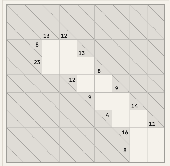
Puzzle 6 (9×9)
