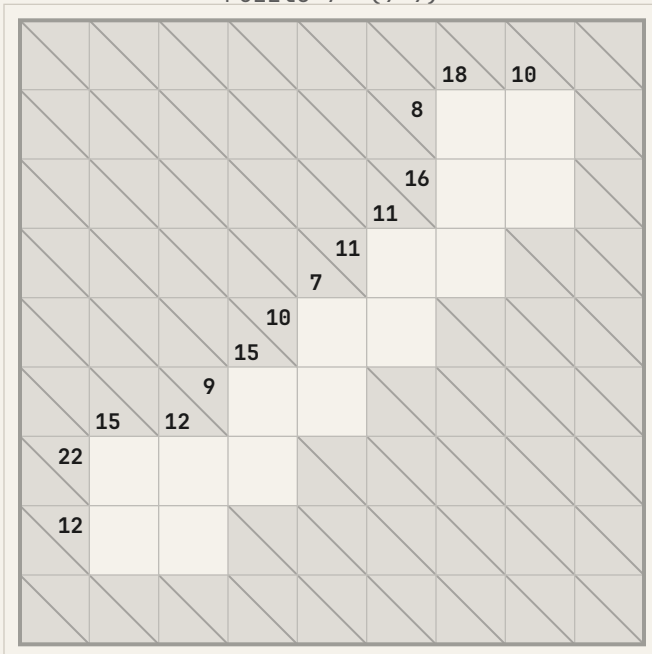
Puzzle 7 (9×9)
