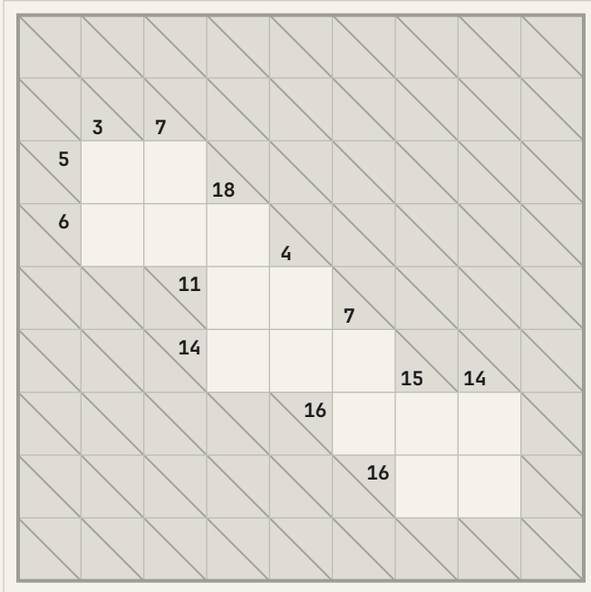
Puzzle 5 (9×9)
