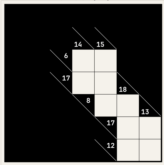
Puzzle 3 (7×7)
