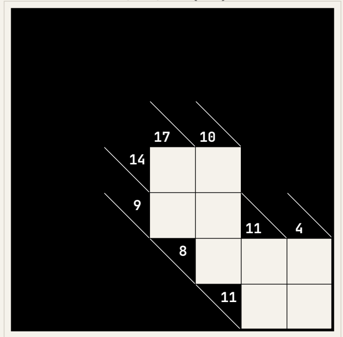
Puzzle 4 (7×7)
