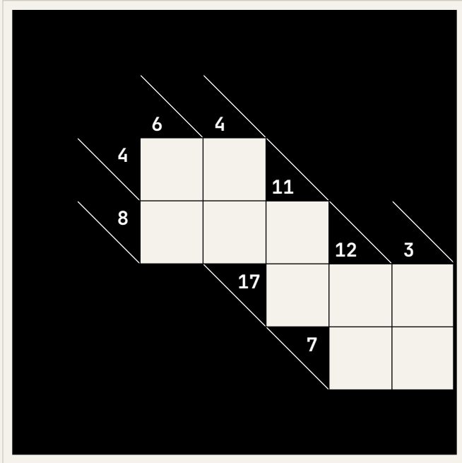
Puzzle 1 (7×7)
