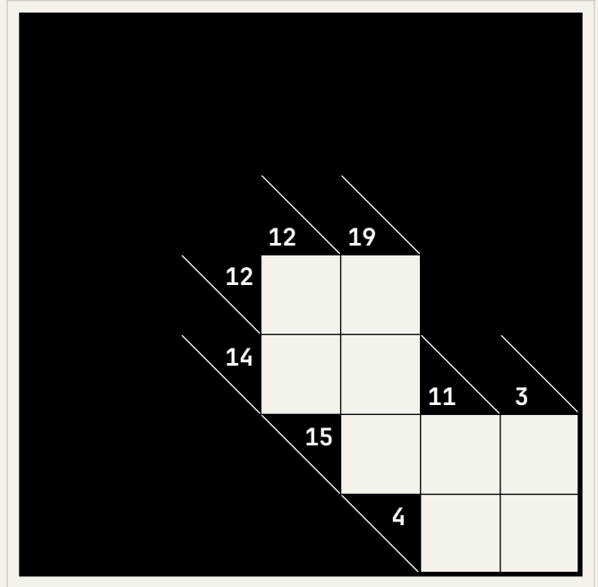
Puzzle 2 (7×7)
