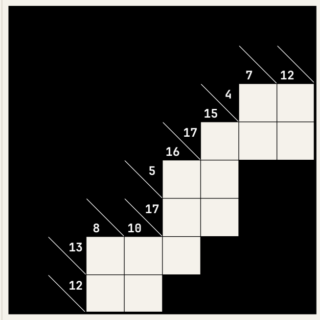
Puzzle 1 (8x8)
