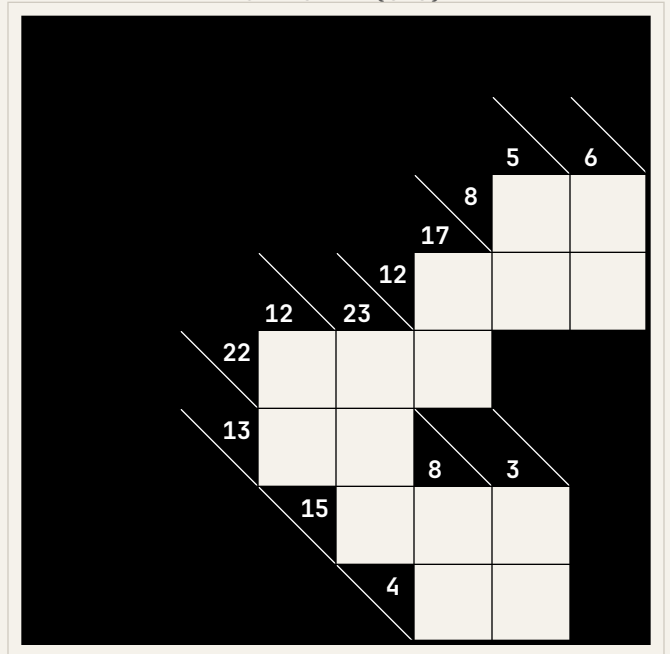
Puzzle 4 (8x8)
