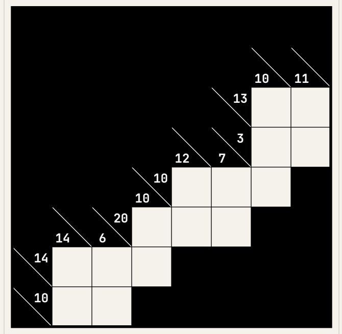
Puzzle 2 (8x8)
