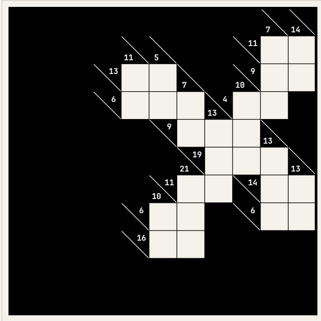
Puzzle 1 (11×11)
