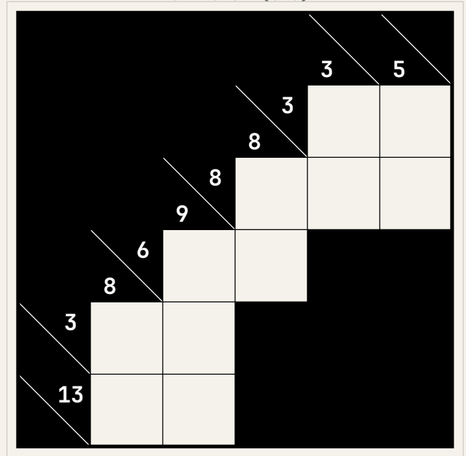
Puzzle 8 (6×6)
