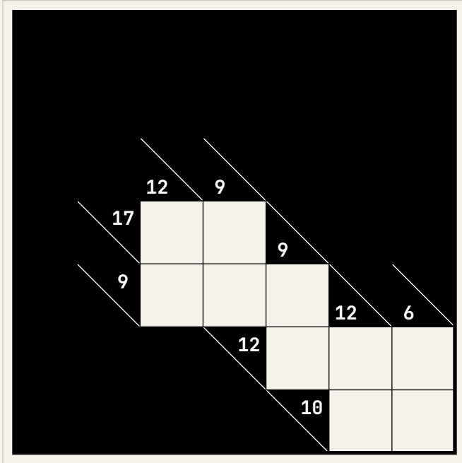
Puzzle 5 (7×7)
