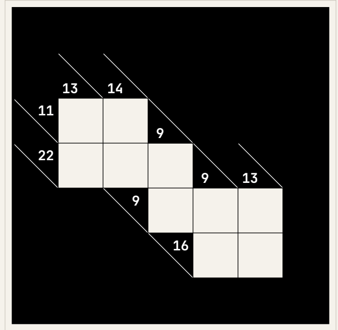
Puzzle 6 (7×7)
