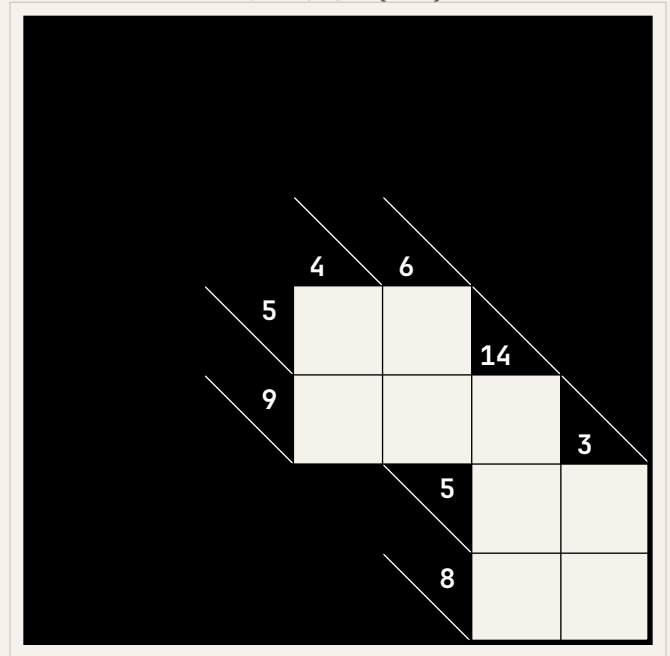
Puzzle 8 (7×7)
