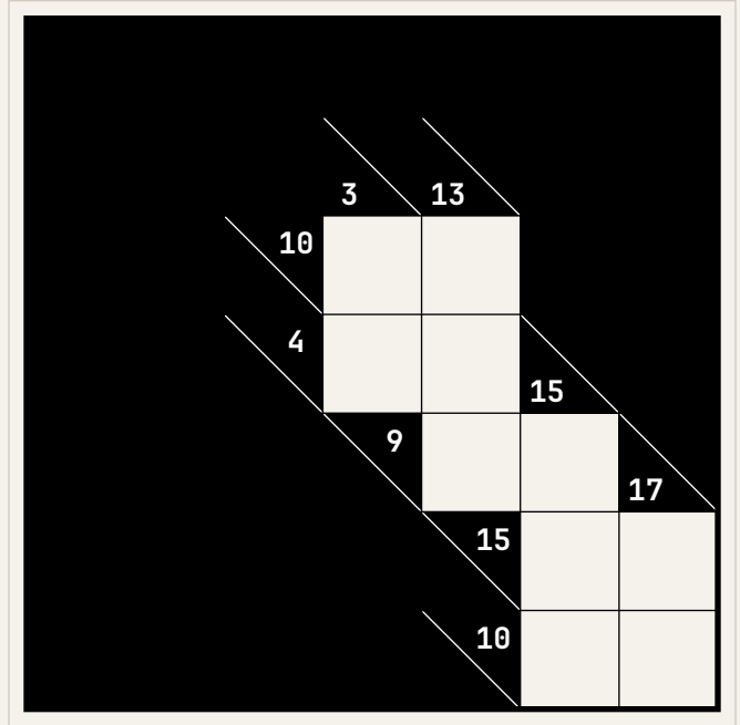
Puzzle 6 (7×7)
