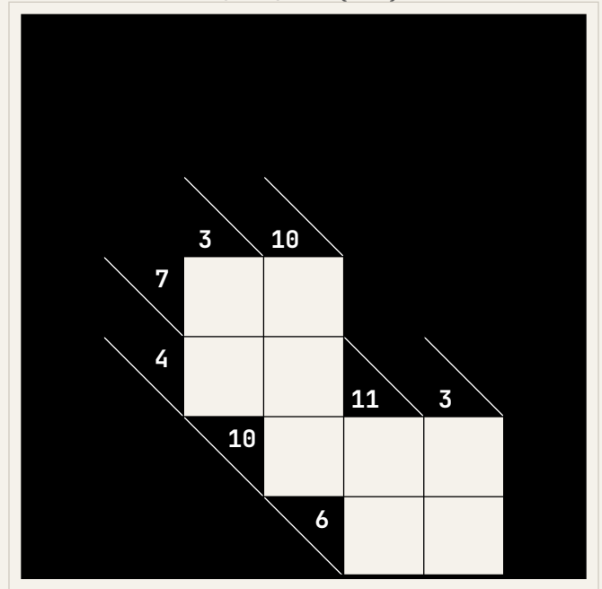
Puzzle 4 (7×7)
