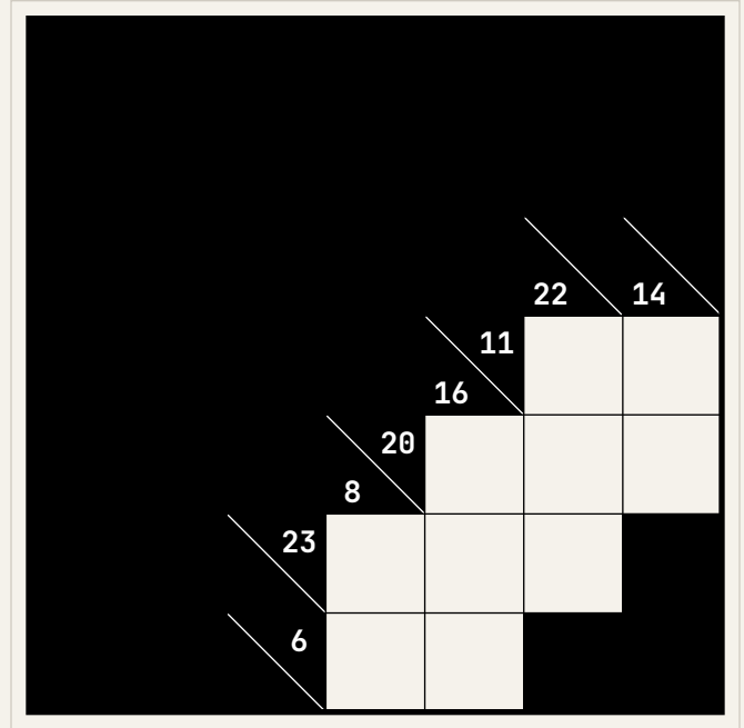
Puzzle 2 (7×7)
