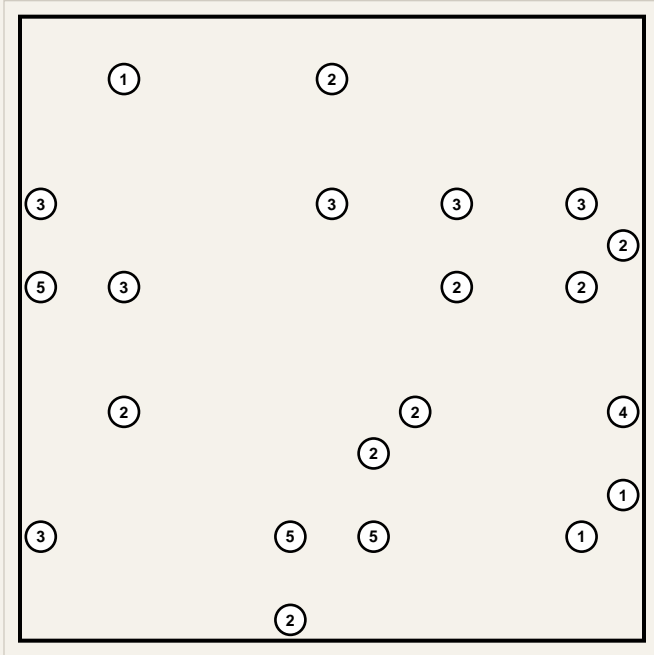
Puzzle 5 (15×15)
